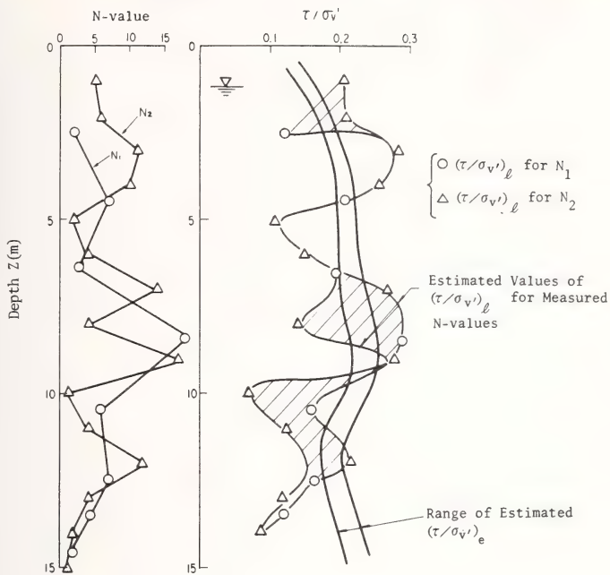
Fig. 31 Comparison of (\tau / \sigma_v')_l of Clean Sand for Measured N-values with (\tau / \sigma_v')_e
